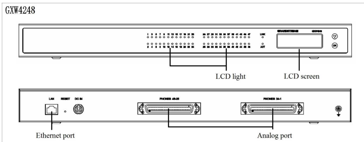
FIGURE 1: DIAGRAM OF GXW4216/24/32/48 PANEL
