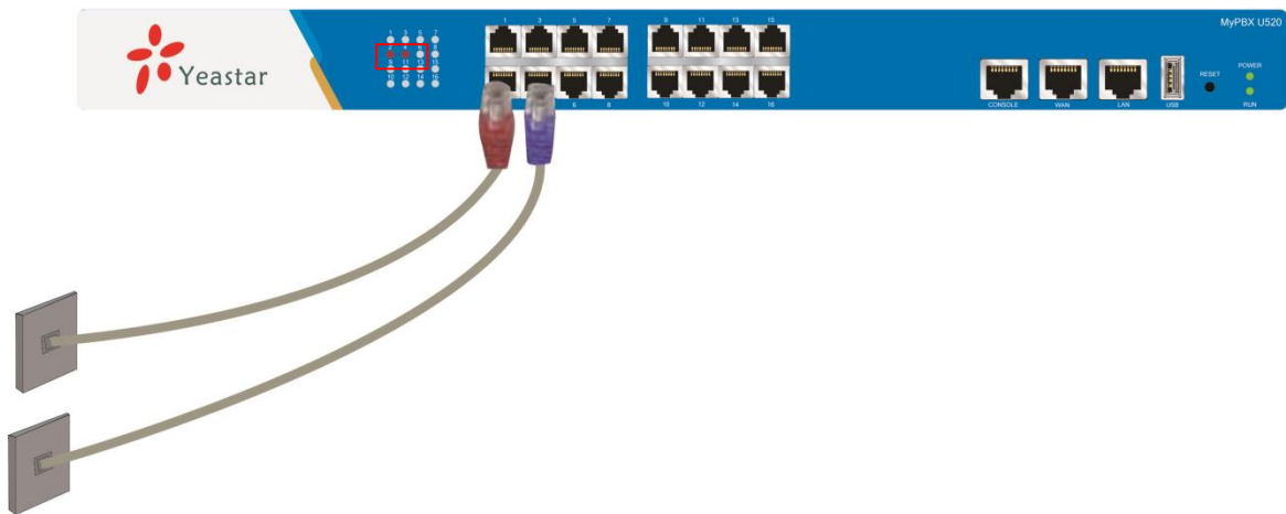
Figure 3-1 Connection of FXO ports and status LED
