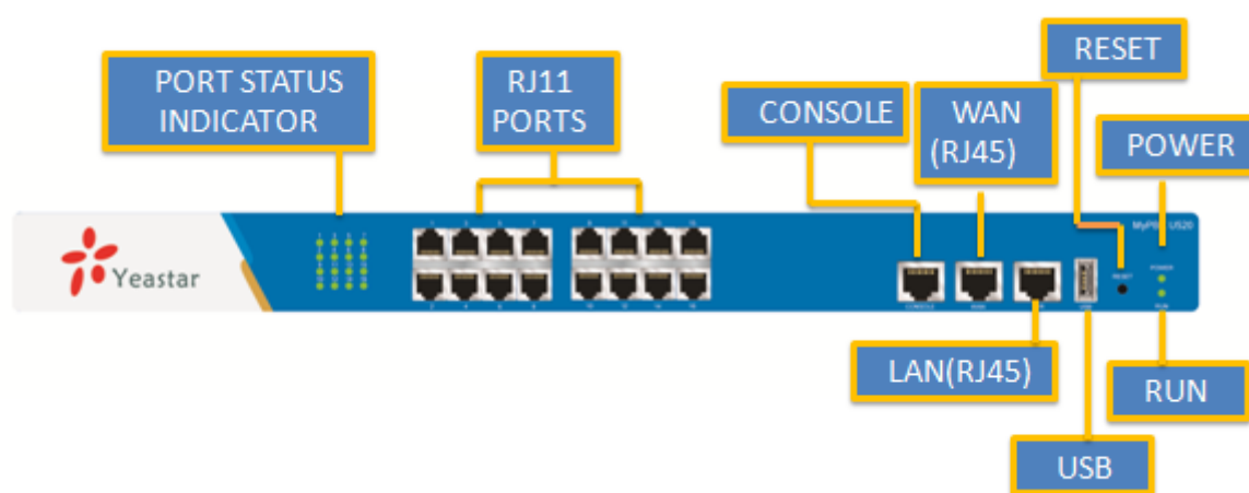
Figure 2-2 MyPBX U500 Front Panel
