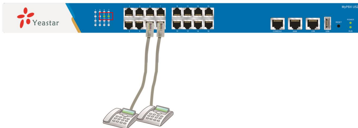
Figure 3-5 Connection of FXS ports and Status LED
